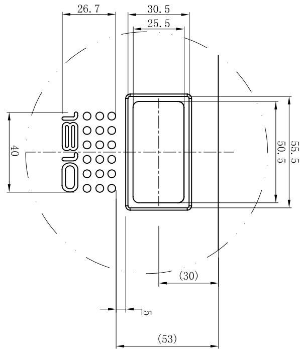
VIEW A
